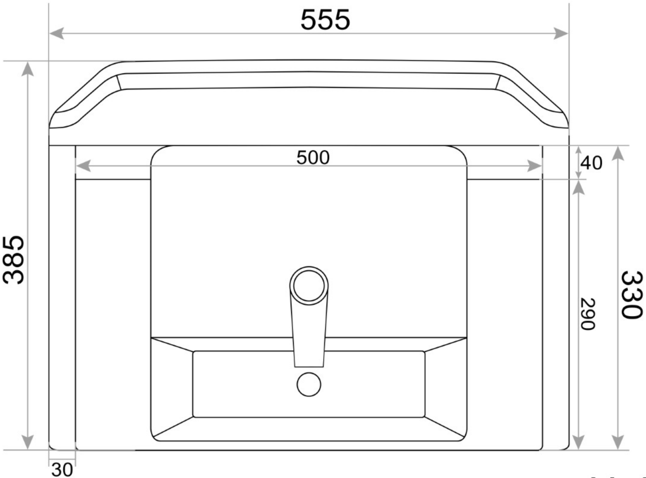
BACK VIEW
